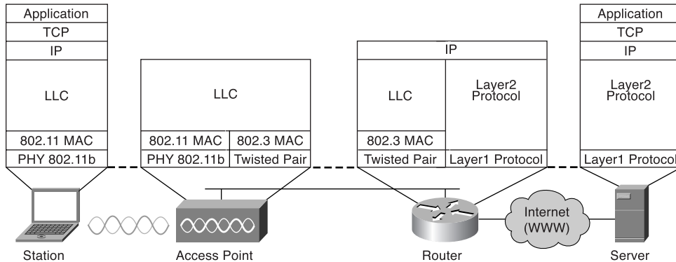
Figure 14-4 802.11 Protocol Stack
